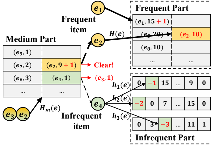
Fig. 2. Data Structure of JoinSketch.
