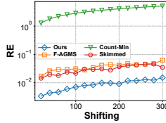
Fig. 5. Impact of dataset correlation.
