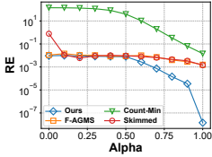
Fig. 4. Impact of dataset skewness.
