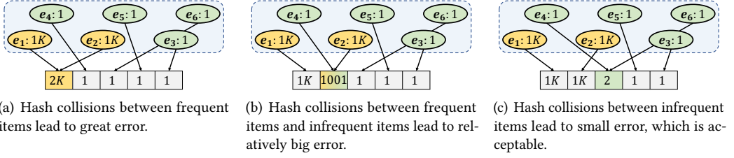
Fig. 1. Types of Hash Collisions.
