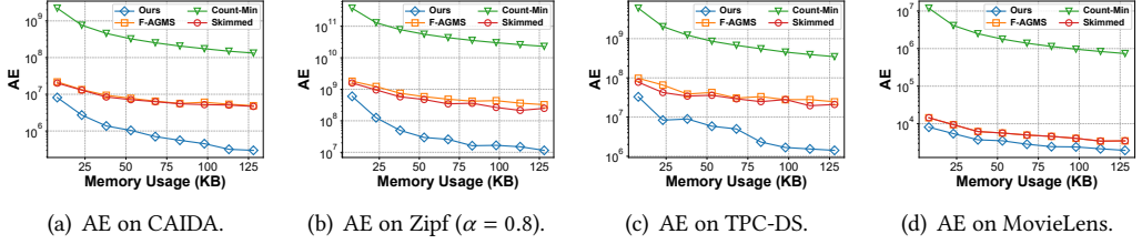
Fig. 3. AE on various datasets.
