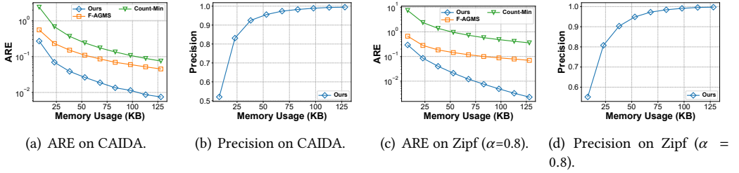
Fig. 10. Accuracy of finding frequent items.
