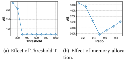
Fig. 12. Impact of different parameters of JoinSketch.
