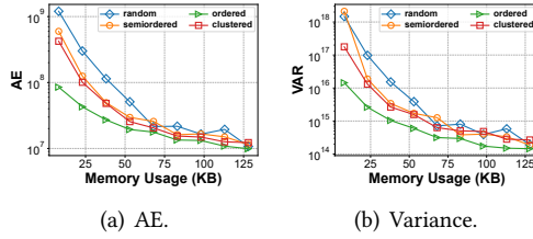
Fig. 8. Impact of data arrival orders.
